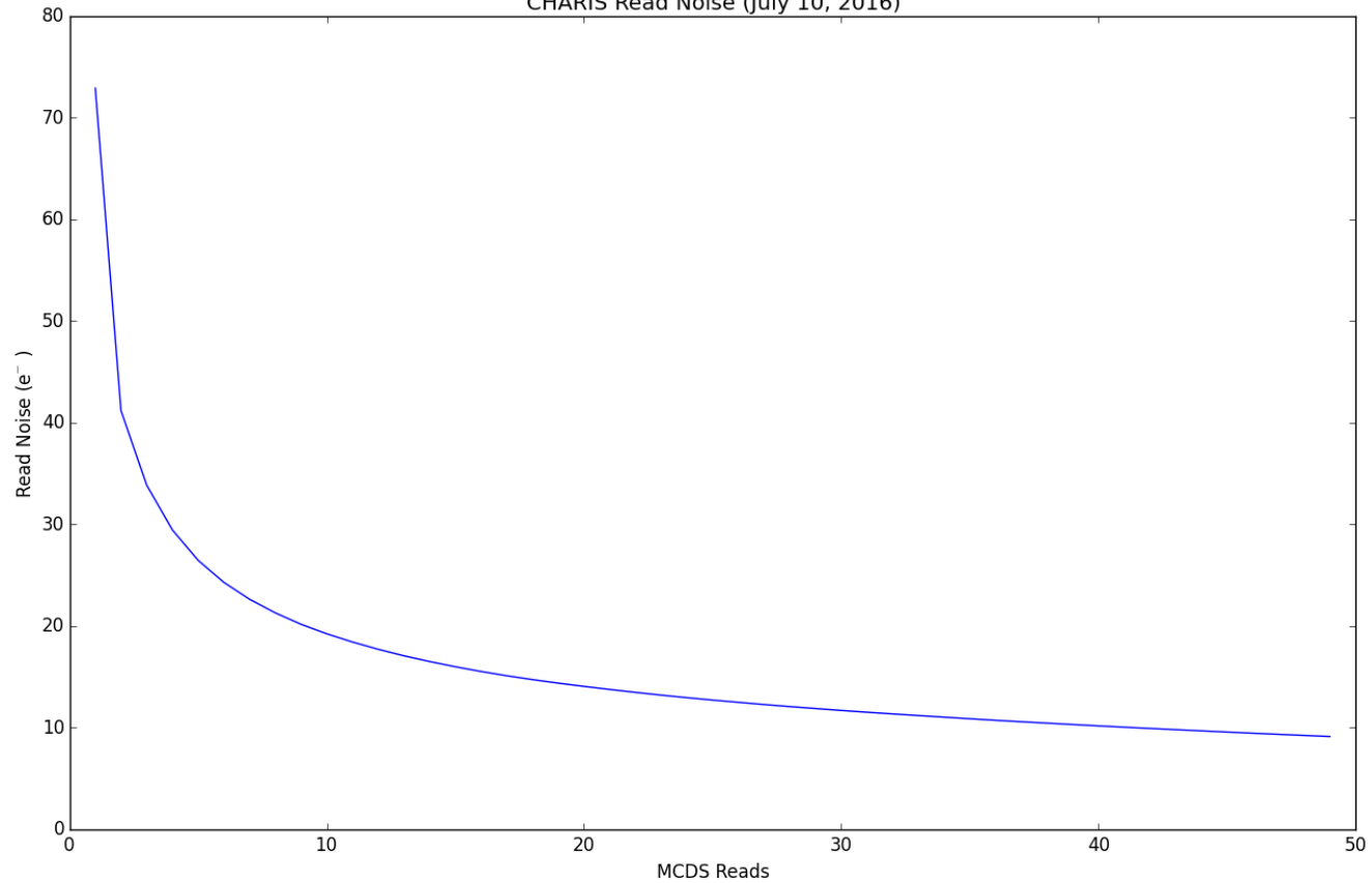
CHARIS Read Noise (July 10, 2016)
